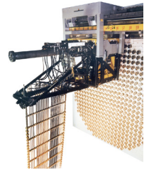
Fuelling Machine
