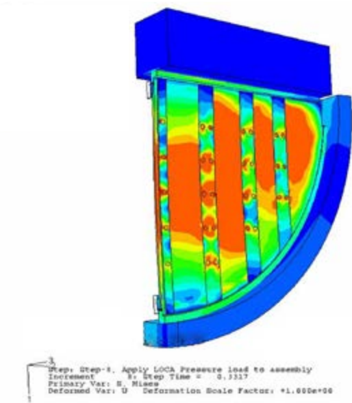
Elastic-plastic analysis a vessel divider plate under pipe rupture load
